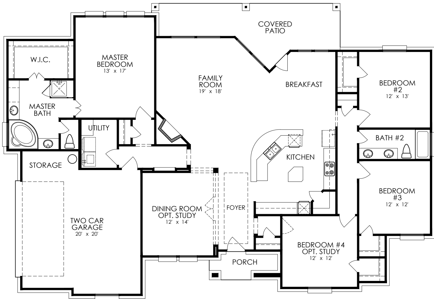
FLOOR PLAN
